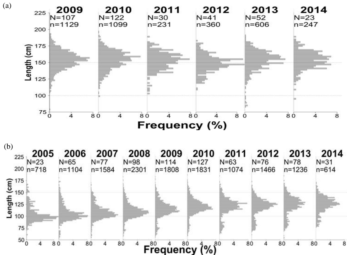
Figure 1: Annual length-frequency distributions for: (a) Dissostichus mawsoni , and (b) D. eleginoides in Subarea 48.4. The number of hauls from which fish were measured (N) and the number of fish measured (n) in each year are provided. Note: length-frequency distributions are only presented for those years in which the number of fish measured was >150.
