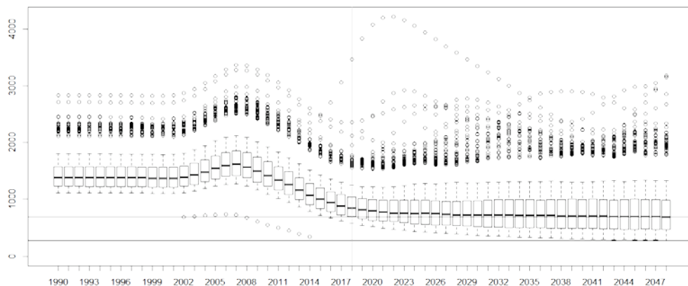
Figure A2: Dissostichus eleginoides in Subarea 48.4: Estimated spawning stock biomass based on a 35-year projection at a constant yield of 45 tonnes. Boxes show median and 25th and 75th percentiles. Whiskers extend to the 5th and 95th percentiles.
