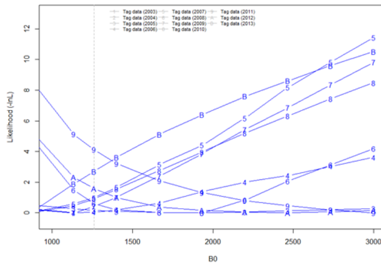
Figure A1: Dissostichus eleginoides in Subarea 48.4: Likelihood profiles for values of B_0 . Negative log likelihood values have been rescaled to have minimum 0 for each dataset. Vertical line indicates the overall MPD estimate of B_0 .
