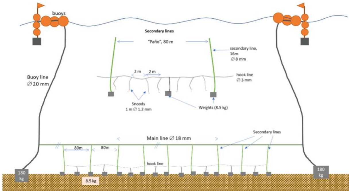
Figure B.5: Details of the Spanish longline proposed for fishing in the Subarea 48.2. Diagram as required in CM 10-02.
